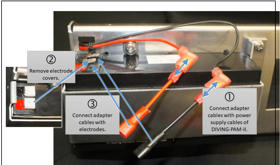
Figure 5: Connecting the Battery
