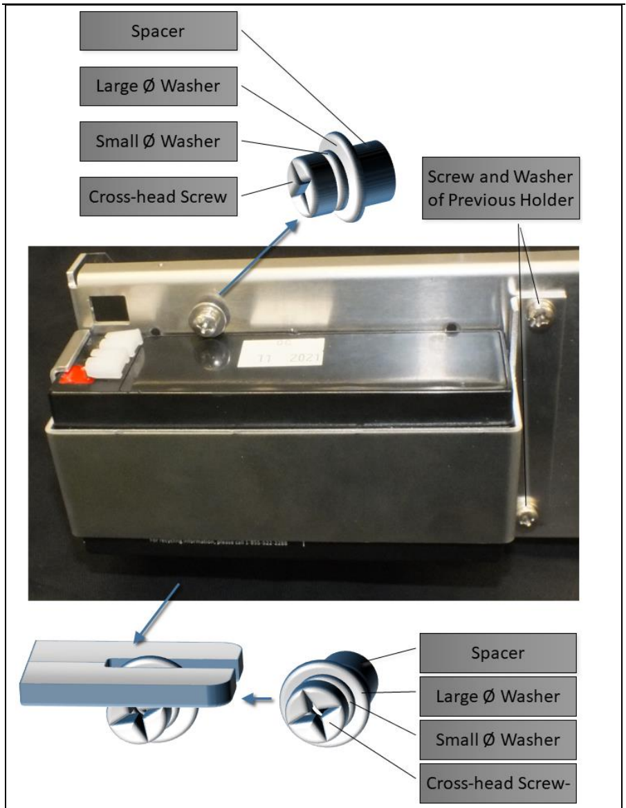
Figure 4: Mounting of Battery Holder
